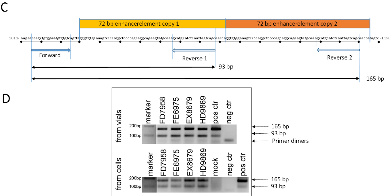
Figures 3C & 3D. Polymerase chain reaction (PCR) reveals residual DNA of the 72 bp SV40 element in the modRNA. C: Map of the SV40 promoter/enhancer region shows the two copies of the 72bp element that result in the two amplicons visible in the PCR due to two binding-sites of the reverse primer in combination with the single binding-site of the forward primer. D: Additional PCR for the SV40 promoter/enhancer (same PCR conditions as in Figure 3B except for a longer runtime) in order to better separate and visualize the two amplicons at 165 bp and 93 bp.
