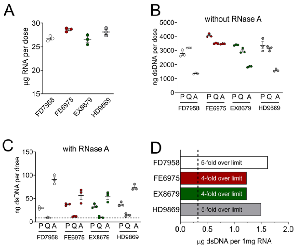
Figure 2. RNA and DNA content of different BNT162b2 biologicals. A: Levels of modRNA per clinical dose were determined in vials by Qubit. n=3 , \text{mean} \pm \text{SEM} . B-C: Levels of double-stranded (ds) DNA per clinical dose in different vials measured by Picco Green (P), Qubit (Q) and AccuBlue (A) without RNase A (Figure B) and with RNase A (C) treatment. The dashed line shows the EMA limit of allowed dsDNA levels in biologicals. n=3 , \text{mean} \pm \text{SEM} . D: Ratio between the dsDNA and RNA content of the vials and the limit that was exceeded according to the EMA regulation of 0.33mg dsDNA per 1mg RNA (dashed line). SEM, standard error of the mean.
