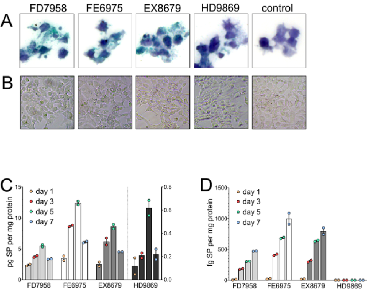
Figure 1. Spike protein expression in HEK293 cells after transfection with BNT162b2 biologicals. A: Staining of spike proteins in cells transfected with different lots visualized in green color by immunohistochemistry. Non-transfected cells (control) show no staining. Hematoxylin serves as nuclei counterstain. B: Brightfield microscopy of transfected HEK293 cells with different lots show an accumulation of intracellular vesicle formation. C: Quantification of intracellular spike protein (SP) concentrations over time measured by ELISA. n=2; mean+SEM. D: Quantification of secreted spike protein (SP) levels over time measured by ELISA. For lot HD9869, secreted spike protein concentration was below the detection limit. n=2; mean+SEM. The negative control showed no spike protein content in the cell lysate and cell supernatant. SEM, standard error of the mean.
