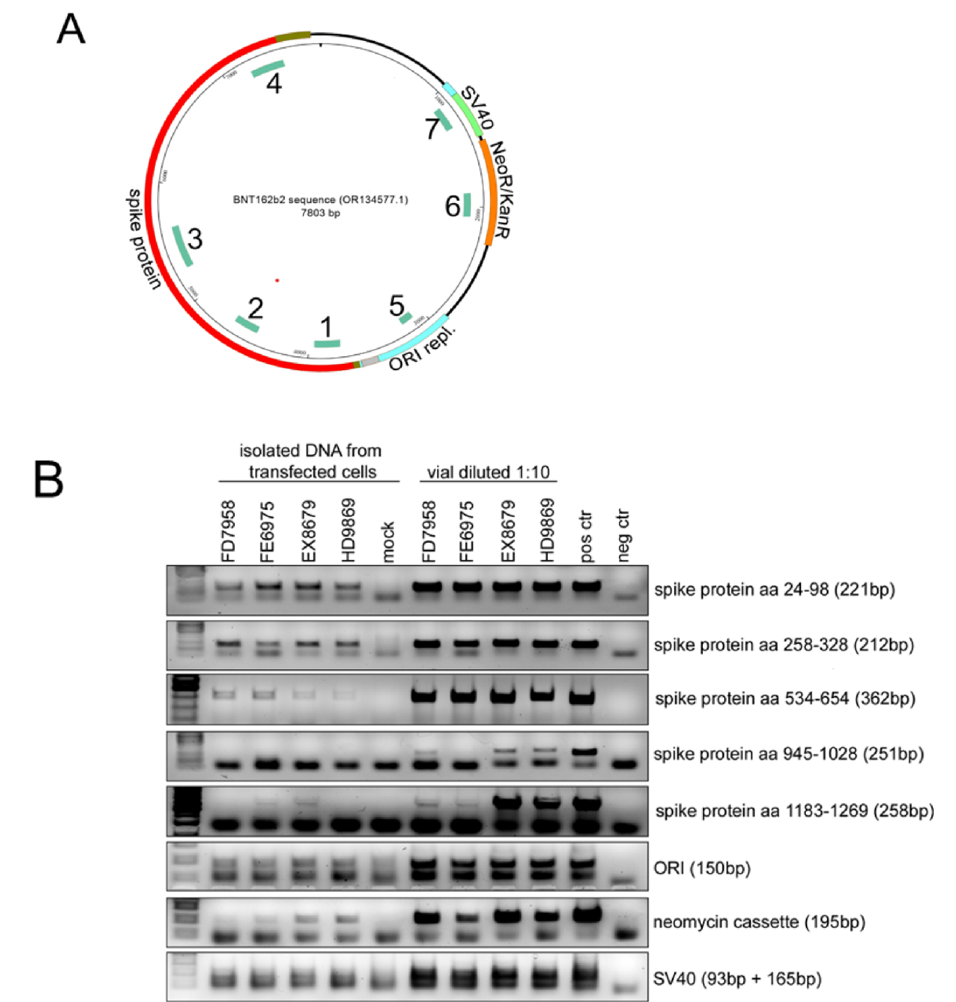
Figures 3A & 3B. Polymerase chain reaction (PCR) reveals residual DNA of the complete plasmid used in the modRNA production process. A: Schematic representation of the DNA plasmid used by BioNTech as a template for modRNA production. Specific sequences (SV40 promoter/enhancer; neomycin resistant cassette, ORI replicon, spike protein) are highlighted in color, as are the sequences used to detect these genes, which are numbered from 1 to 7. B: Visualized DNA fragments after PCR of the indicated sequences (Figure A, 1-7) show the detection of all genes from the DNA plasmid in the vials (right, diluted 1:10 before loading to the PCR) and in plasmid preparations from cells transfected with these biologicals (left). Mock stands for non-transfected cells as negative control for the left part and water as negative control for the right part. Lot GH9715 served as positive control.
